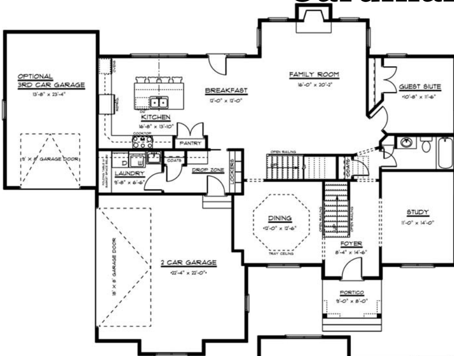
FIRST FLOOR PLANS
